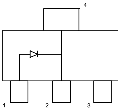
SOT-223 Pin Out Configuration
